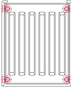
4 Giriş-Çıkışlı 4 Holes Connection
